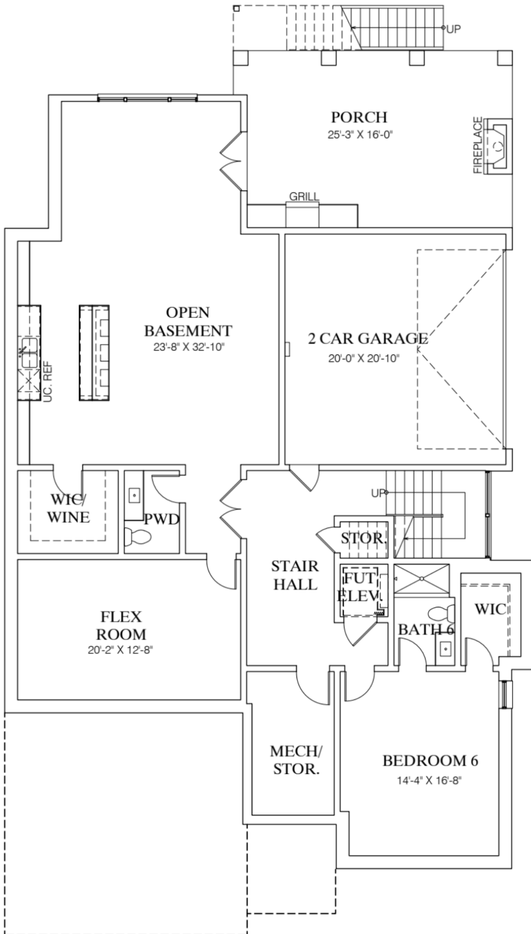
BASEMENT PLAN
