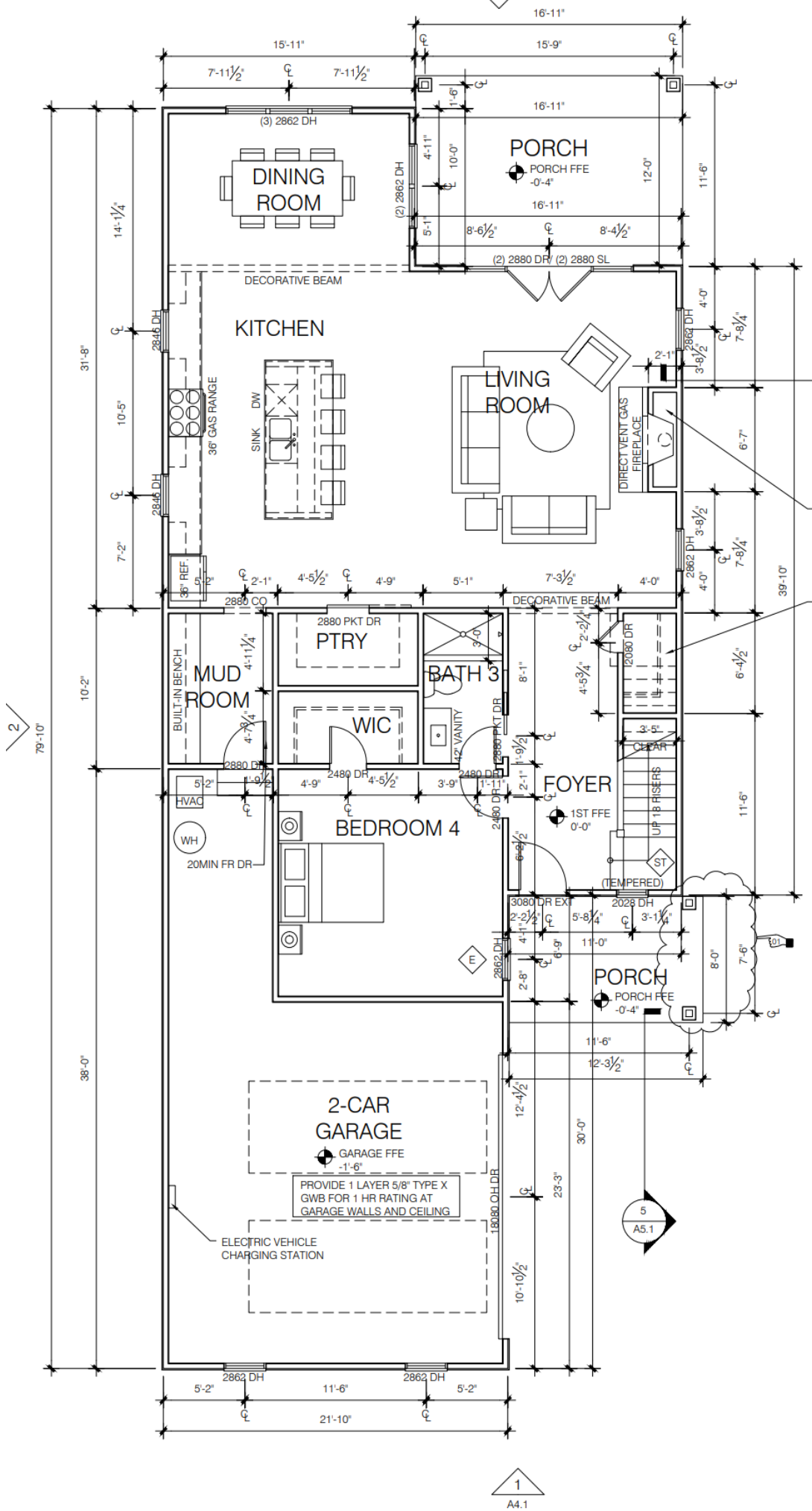
1 floor plan - 1st floor
