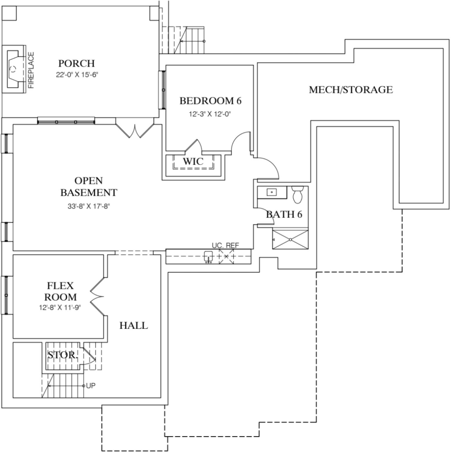
BASEMENT PLAN
