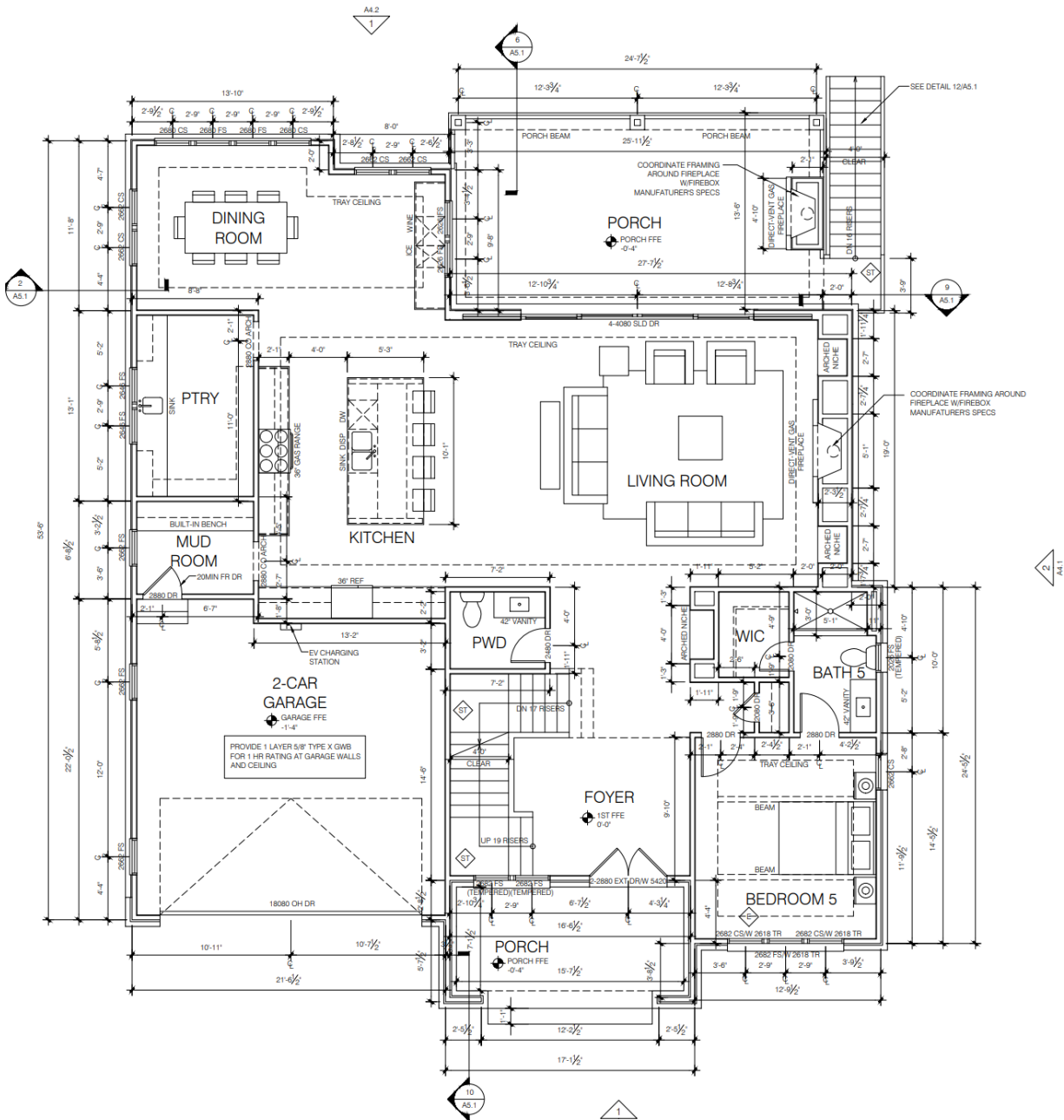
1 floor plan - 1st floor A4.1 SCALE: 1/4" = 1'-0"
