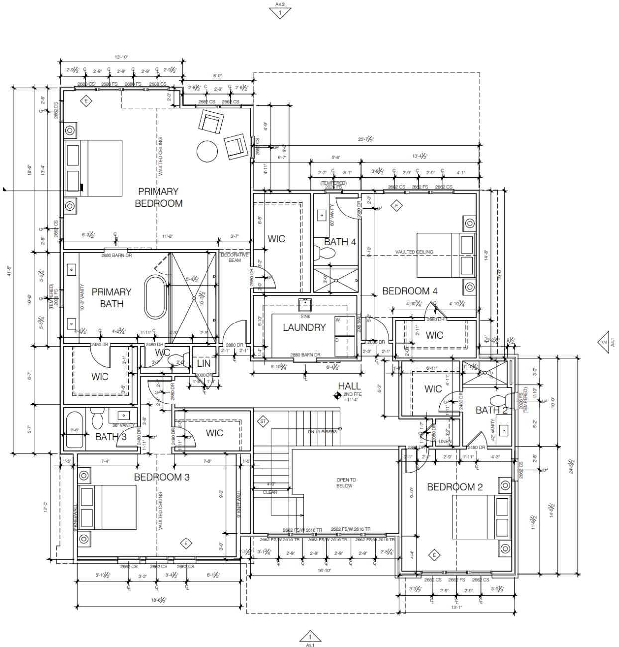
1 floor plan - 2nd floor A2.2 SCALE: 1/4" = 1'-0"
